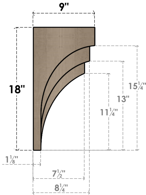
SIDE PROFILE
